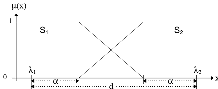
Figure 4. Defining the crispness of a partitioning.
