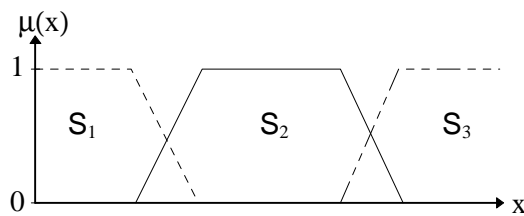
Figure 1. Typical 1D membership functions.
